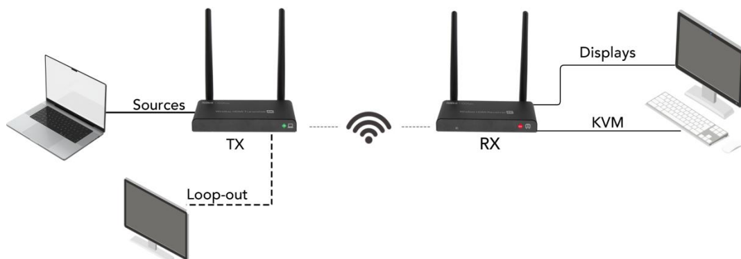
ASK plus p2p System Connection Diagram
