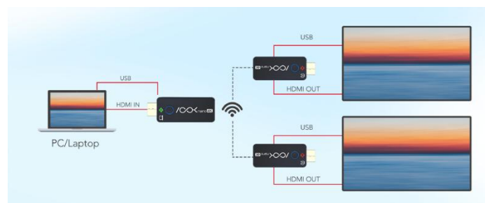
ASK nano System Connection Diagram 1
