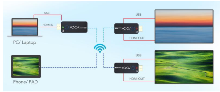
ASK nano System Connection Diagram 2
