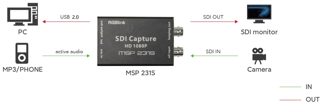
MSP 231S System Connection Diagram
